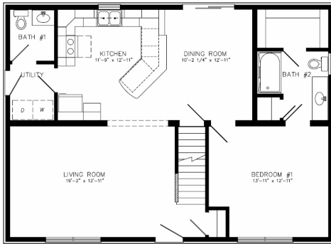
27'-6" X 38'-0" 1045 SQ/FT
